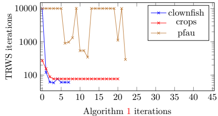
Figure 3. Iterations needed by TRWS [15] in Algorithm 1 for three Potts instances.
