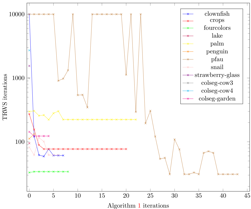
Figure 1. Iterations needed by TRWS [10] by our Algorithm for Potts-datasets.
