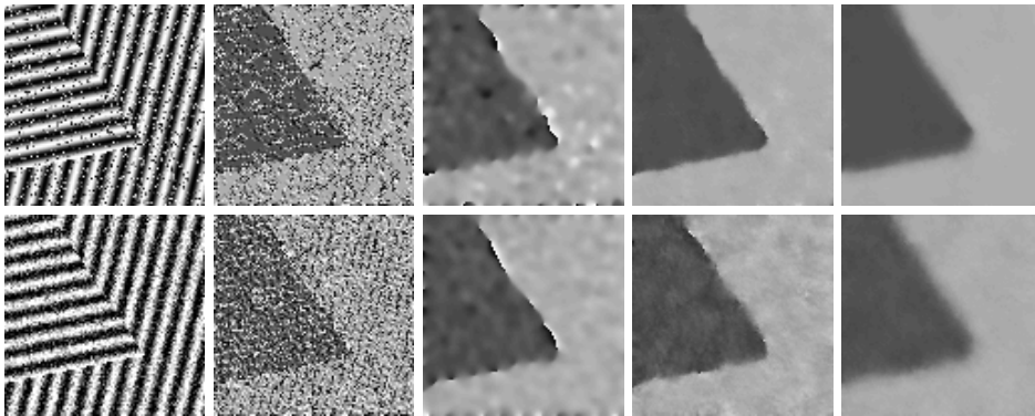
Figure 6: Top, left to right: (a) Test image with 20% impulse noise. (b) Orientation field of (a). (c) Structure tensor orientation obtained by Gaussian smoothing of the outer product matrices with standard deviation 19. (d) Same after median filtering with Frobenius norm and disk-shaped structure element of diameter 9. (e) Median filtering of (a) with Frobenius norm and disk-shaped structure element of diameter 9. Bottom, left to right: (f) Test image perturbed by Gaussian noise of standard deviation 0.2 (where grey-values vary between 0 and 1). (g) Orientation field of (f). (h) Structure tensor orientation as in (c). (i) Median filtering as in (d). (k) Median filtering as in (e). From [35].
