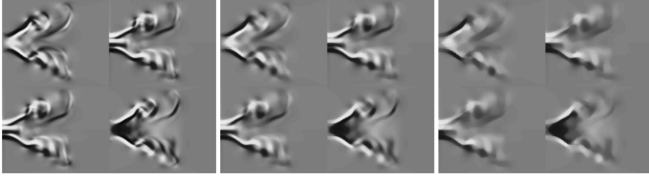
Figure 3: Frobenius median filtering of a tensor field containing indefinite matrices. The data are deformation tensors originating from a fluid dynamics simulation. Left to right: (a) Initial data, 124 \times 101 pixels. (b) 10 iterations, 3 \times 3 stencil. (c) 100 iterations. From [37].
