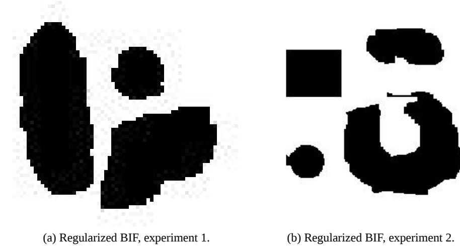
Figure 4. Results obtained by the regularized best inner fit approach (5).
