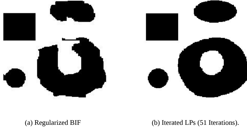
Figure 7. Comparison between regularized BIF and iterating LPs for the second experiment. We terminated the iterated LPs after 51 iterations and set the remaining non-binary pixels (0.07%) to zero in order to obtain a binary solution.
