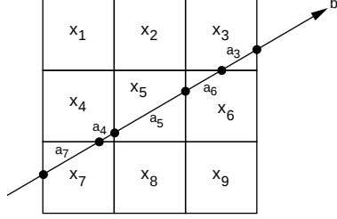
Figure 2. Discretization model leading to the algebraic representation of the reconstruction problem: Ax = b, x \in \{0, 1\}^n .
