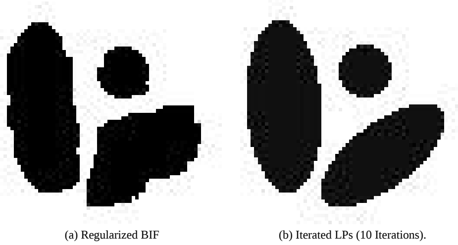
Figure 5. Comparison between the regularized best inner fit approach and our approach proposed in this paper.
