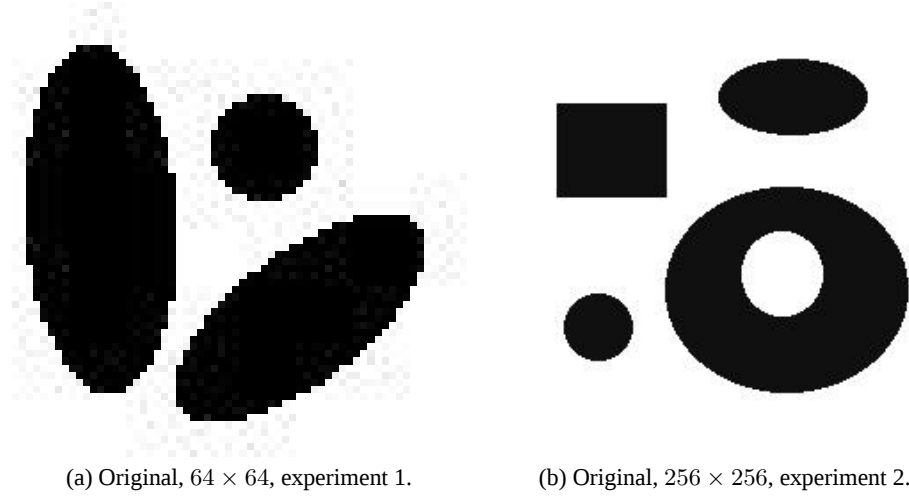
Figure 3. From each image, 3 projections, 0^\circ , 45^\circ , and 90^\circ were taken for setting up the two reconstruction problems used in our evaluation.
