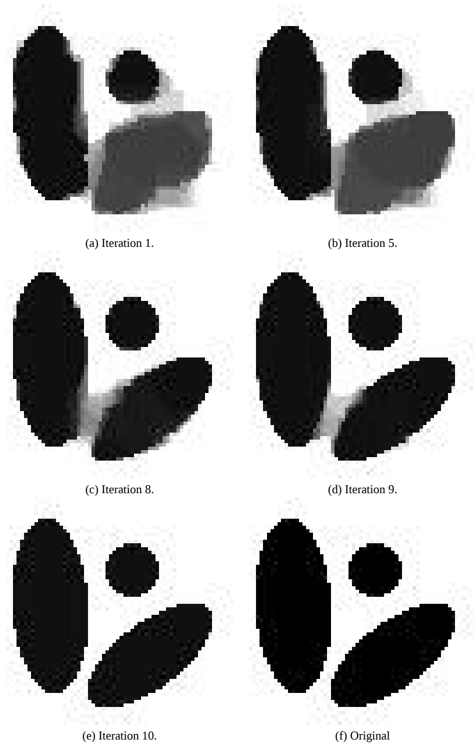
Figure 8. (a)–(e) Results at different iterations of our proposed reconstruction method. The original image is shown in figure 8(f) from which three projections, 0^\circ , 45^\circ , and 90^\circ were taken.
